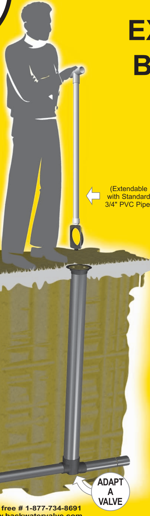
EXTERIOR BACKWATER VALVE INSTALLATION
